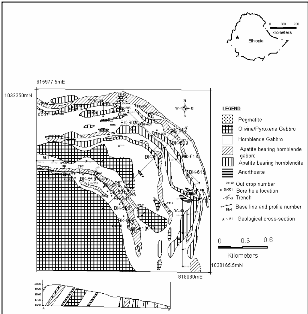
Fig. 1. Geology and Mineralization Map of Soji-Bikilal phosphate Deposit
